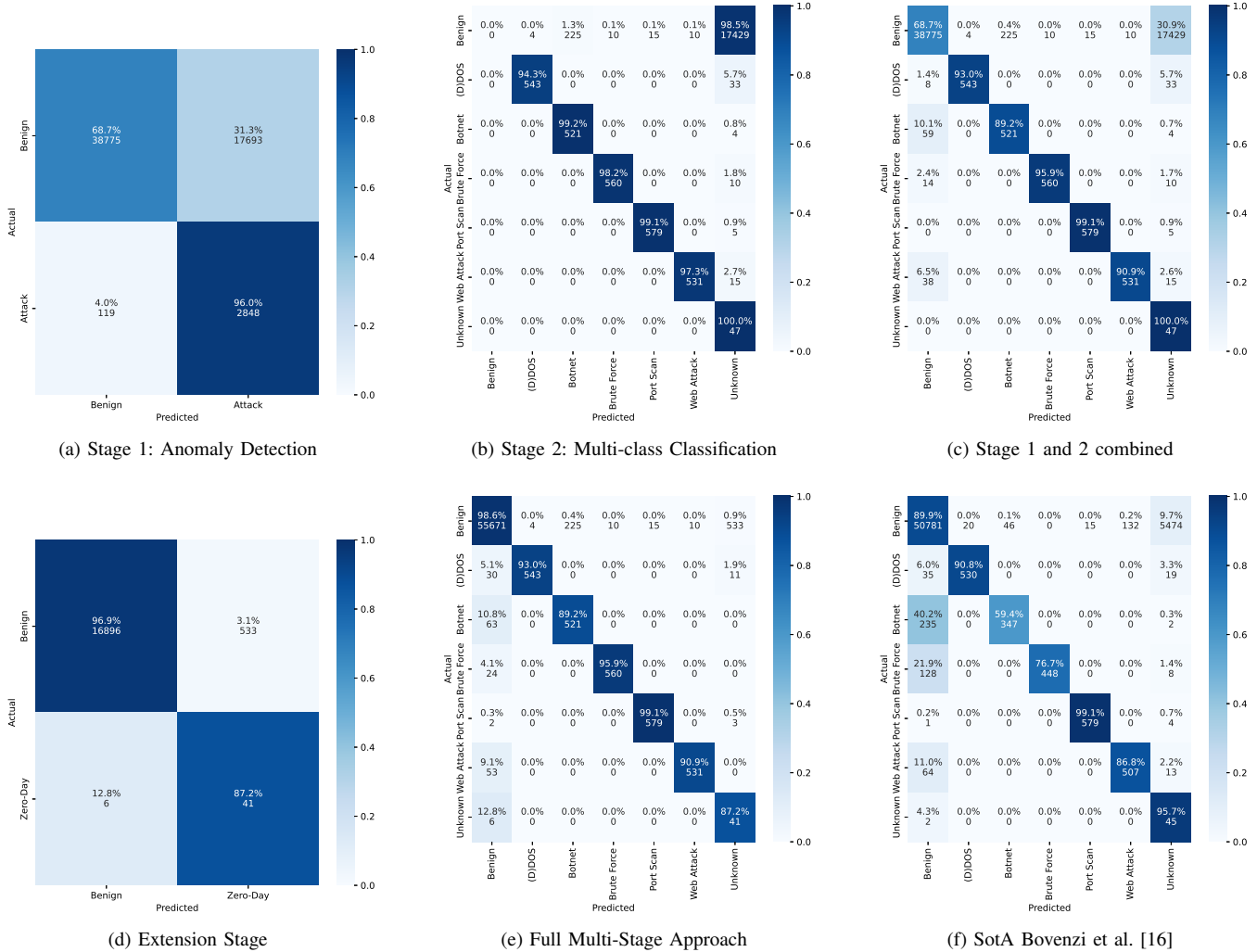
Fig. 4. Confusion Matrices.
