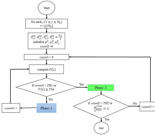
Fig. 3. Flow chart of TPIO.
