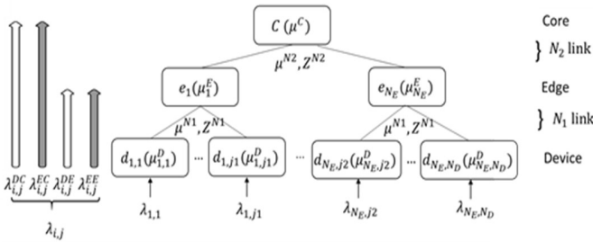
Fig. 1. Three-tier hierarchical MEC-based architecture.
