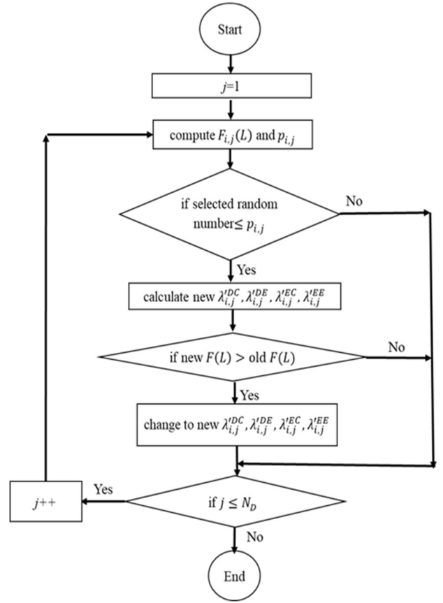
Fig. 4. Flow chart of phase 1.
