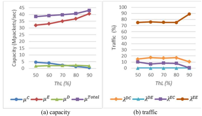
Fig. 11. The effects of ThL .
