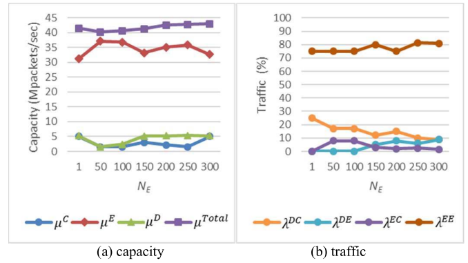
Fig. 9. The effects of the number of edges.
