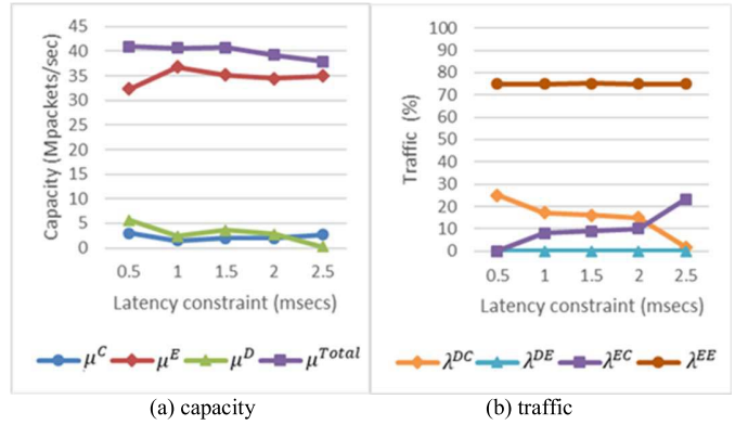
Fig. 10. The effects of latency constraint.
